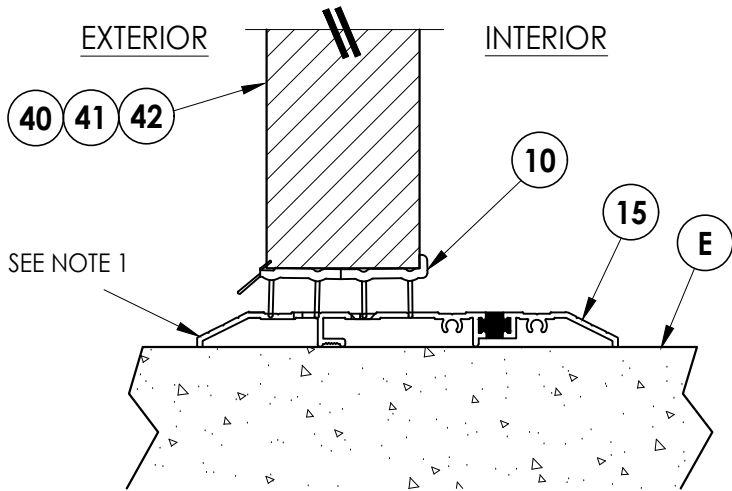
2 VERTICAL CROSS SECTION 7 Public Access Sill
