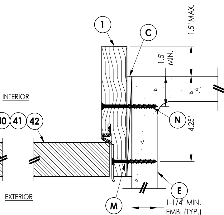
6 HORIZONTAL CROSS SECTION 6 Shown Direct to Masonry 6-9/16" jamb
