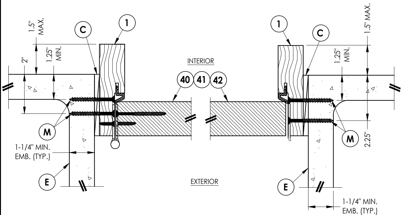
2 HORIZONTAL CROSS SECTION 6 Shown Direct to Masonry 4-9/16" jamb
