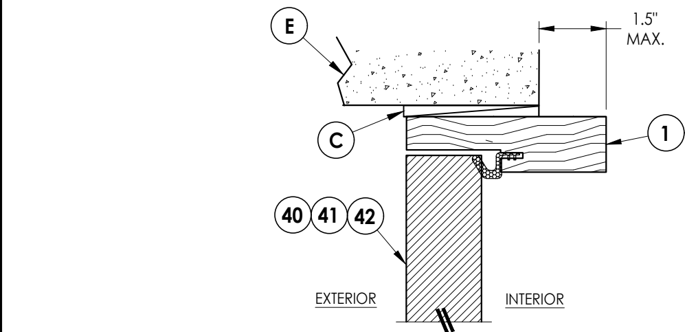
1 VERTICAL CROSS SECTION 6 Shown Direct to Masonry 4-9/16" jamb
