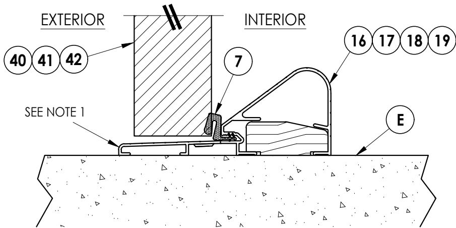
1 VERTICAL CROSS SECTION 7 Outswing Sill (Coastal Sill Shown)
